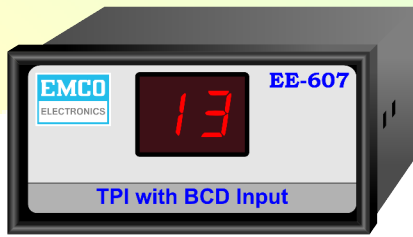
Standard model
