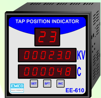
TPI with Counter, Vg. Dis. & 485 Communication
