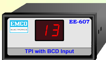
Standard model
